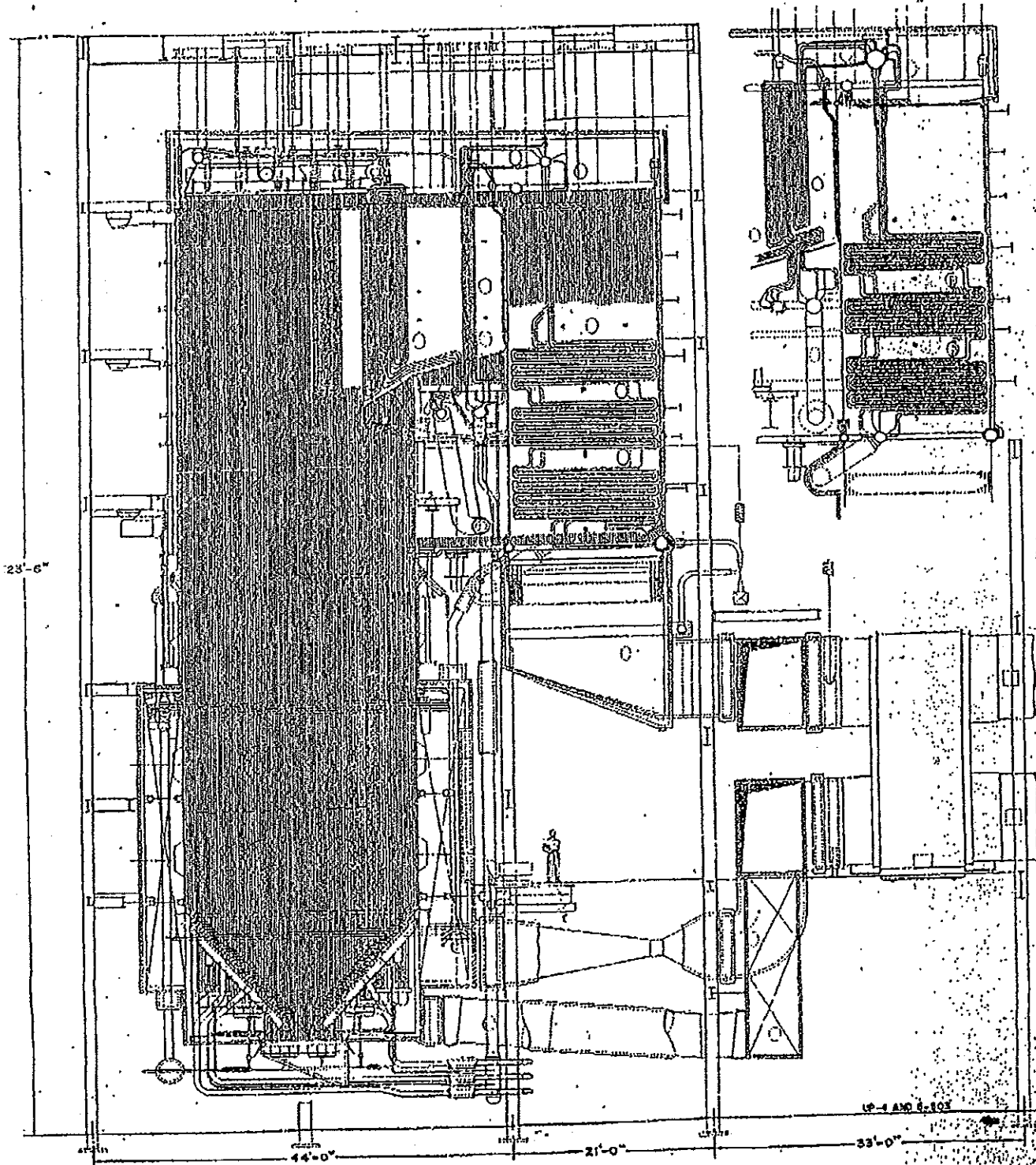
B+W UNIVERSAL PRESSURE BOILERS HUNTINGTON BEACH GEN. STATION UNITS NO. 3 & 4
